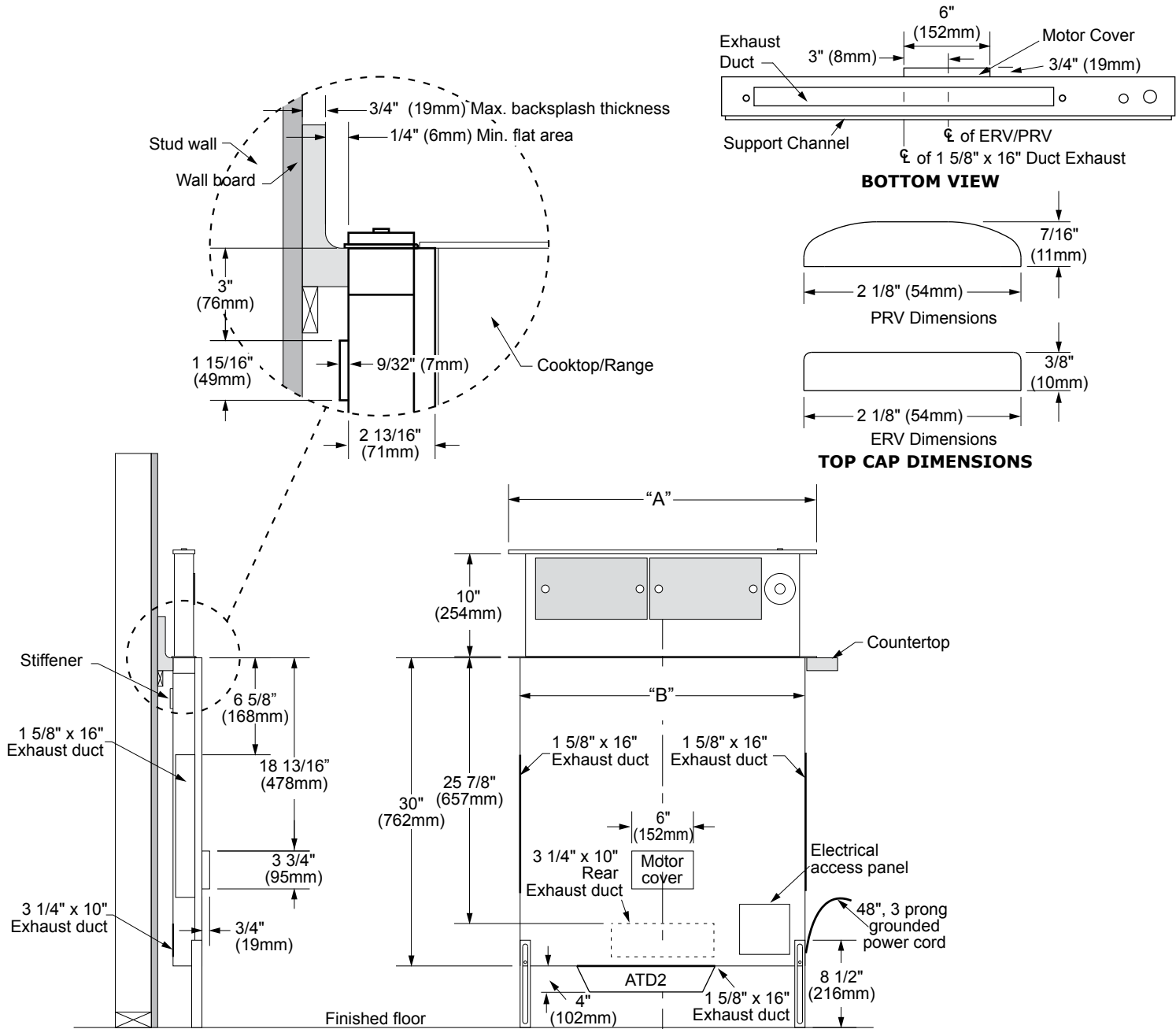
ERV/PRV OVERALL DIMENSIONS
